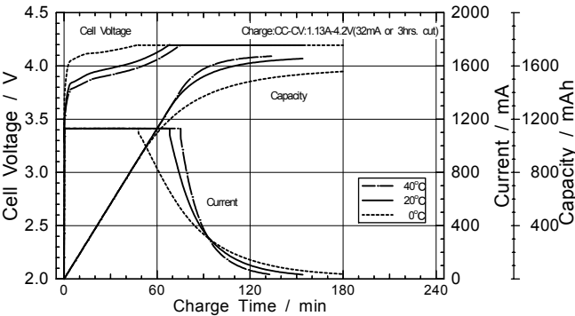
Charge characteristics
